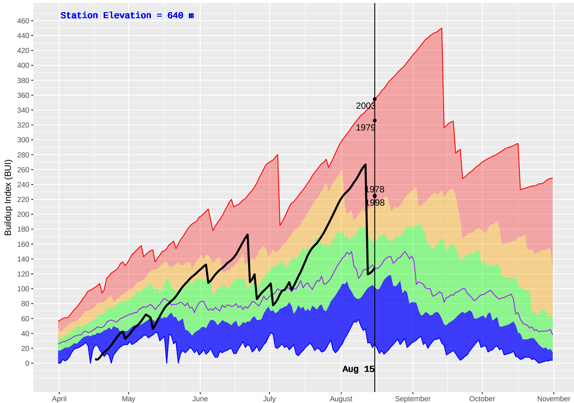
MERRITT HUB (294) : Historical (1978–2016) and Current (2018) Daily Buildup Index (BUI)
